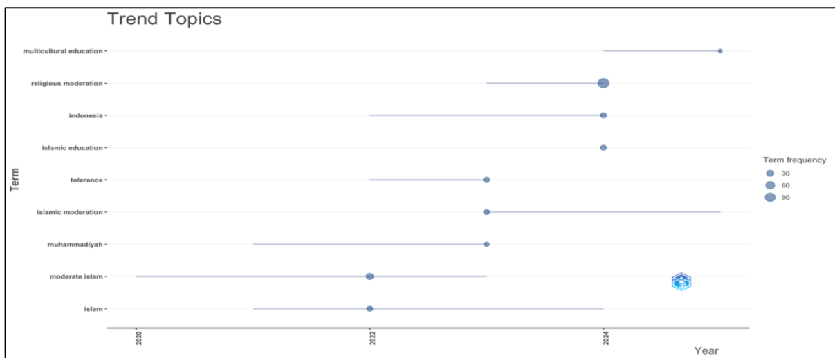
Gambar 10. Trend Topics
