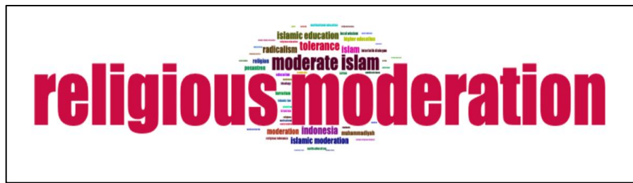
Gambar 8. Word Cloud
