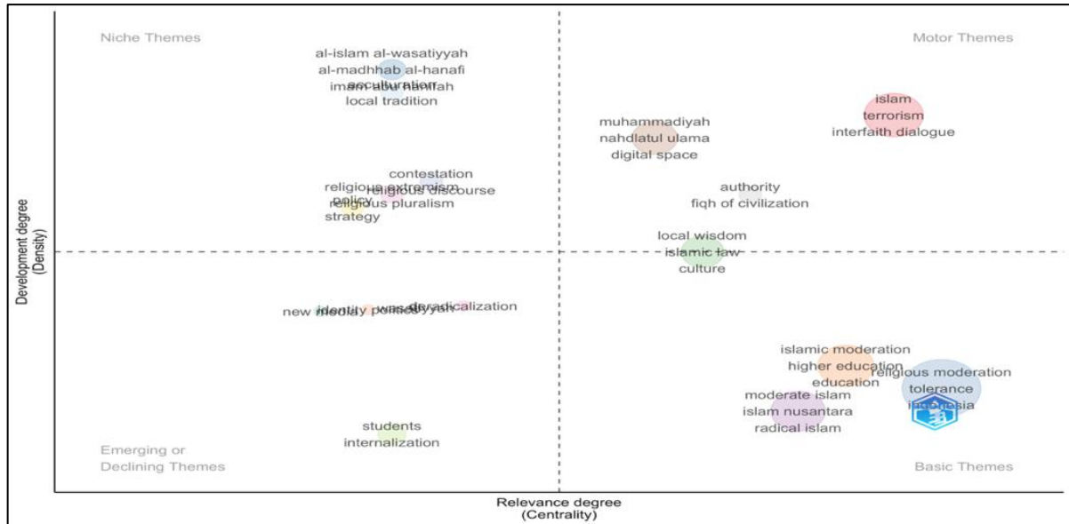
Gambar 11. Thematic Map
